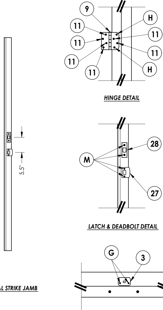
DETAIL 2
