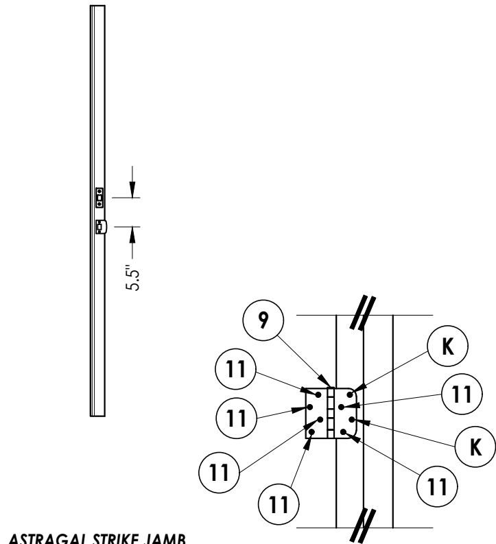
ASTRAGAL STRIKE JAMB
